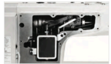
Built-in presser foot lifter
